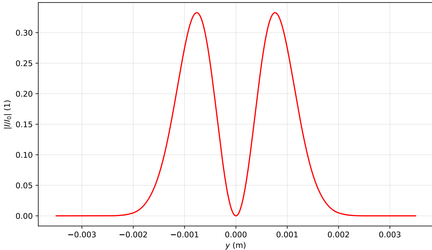
Intensity profile I(x=0, y, z=2.388)/I_0 , P_{in}=0.5P_{cr} , artificial time
